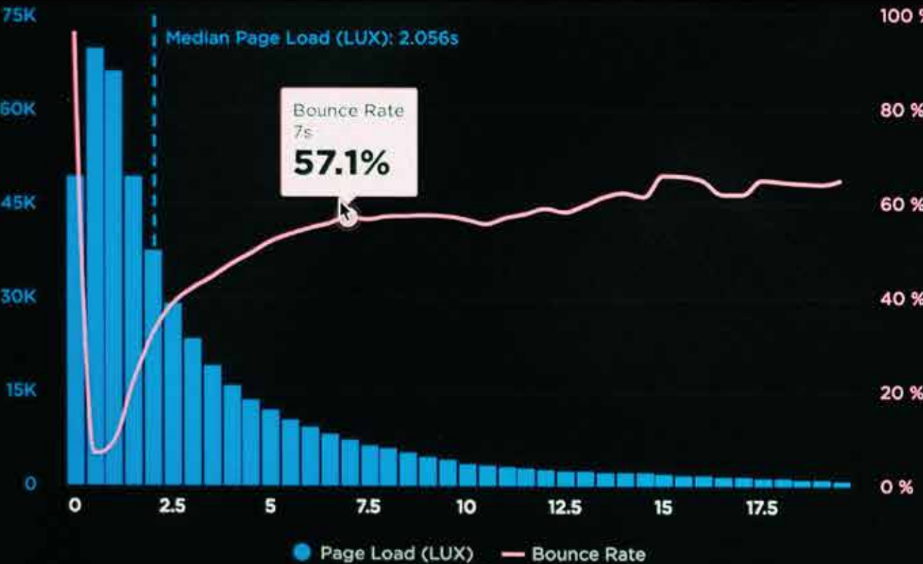
LOAD TIME VS BOUNCE RATE
